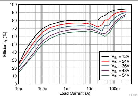
Figure 7-1. Efficiency 5-V Output, Auto Mode
