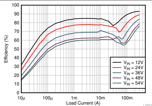
Figure 7-2. Efficiency 5-V Output, Auto Mode
