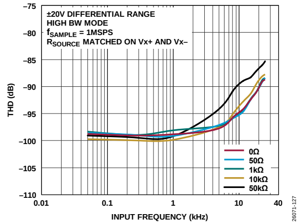
Figure 36. THD vs. Input Frequency for Various Source Impedances, \pm 20\text{ V} Differential Range, High Bandwidth Mode
