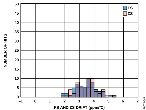
Figure 50. FS and Zero-Scale (ZS) Drift Histogram, 0\text{ V to } 10\text{ V} Single-Ended Range
