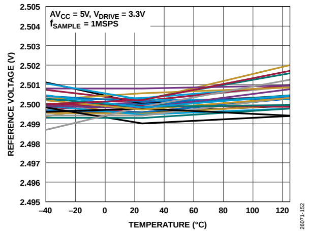
Figure 61. Reference Drift
