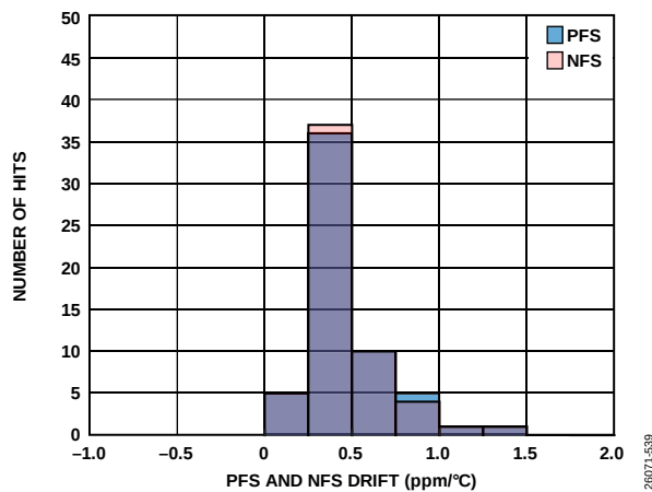
Figure 48. PFS and NFS Drift Histogram, \pm 10\text{ V} Single-Ended Range
