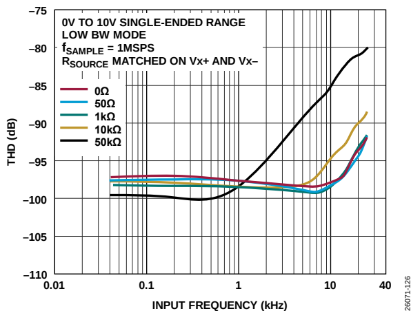
Figure 35. THD vs. Input Frequency for Various Source Impedances, 0\text{ V} to 10\text{ V} Single-Ended Range, Low Bandwidth Mode
