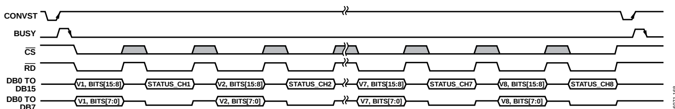
Figure 99. Parallel Interface, ADC Mode with Status Header Enabled
