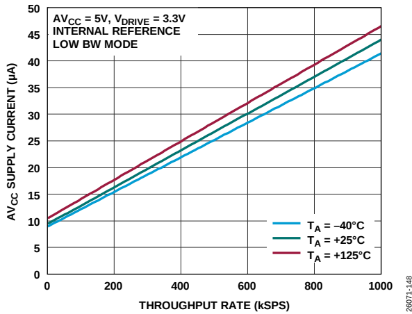
Figure 57. AV_{CC} Supply Current vs. Throughput Rate for Various Temperatures
