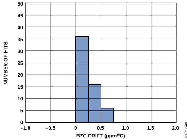
Figure 49. Bipolar Zero Code (BZC) Drift Histogram, \pm 10\text{ V} Single-Ended Range
