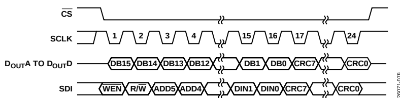
Figure 112. AD7606C-16 Serial Interface, Single Write Command, SDI Clocks in the Address Bit ADD5 to Bit ADD0 and the Register Content Bit DIN7 to Bit DIN0 During the Same Frame, D OUT A Provides Register Content Requested on the Previous Frame
