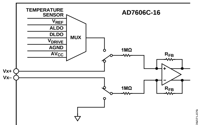
Figure 118. Diagnostic Multiplexer (Channel 1 Shown as an Example) ( R_{FB} = Feedback Resistor)
