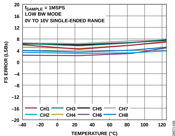
Figure 47. FS Error vs. Temperature, 0\text{ V to } 10\text{ V} Single-Ended Range
