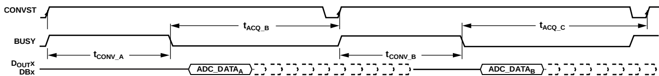
Figure 100. ADC Data Read Can Happen After Conversion and/or During the Following Conversion
