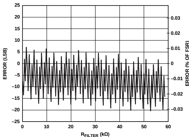
Figure 94. System Error with Gain Calibration Enabled
