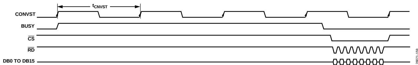
Figure 90. External Oversampling Clock Applied on the CONVST Pin (OSR = 4), Parallel Interface
