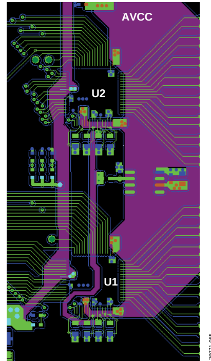
Figure 124. Layout for Multiple AD7606C-16 Devices—Top Layer and Supply Plane Layer
