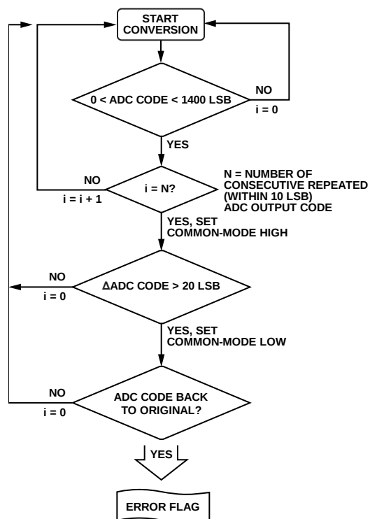
Figure 97. Automatic Analog Input Open Circuit Detect Flowchart
