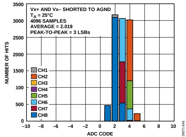
Figure 54. Histogram of Codes, ±20 V Differential Range
