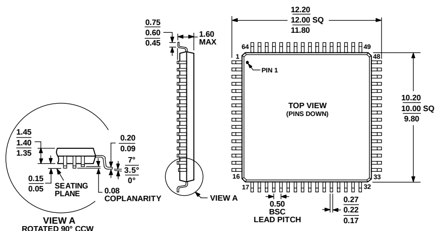
Figure 125. 64-Lead Low Profile Quad Flat Package [LQFP] (ST-64-2)
