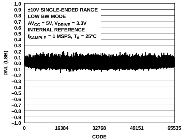
Figure 39. Typical DNL, Low Bandwidth Mode
