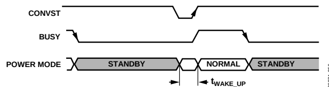
Figure 86. Autostandby Mode Operation
