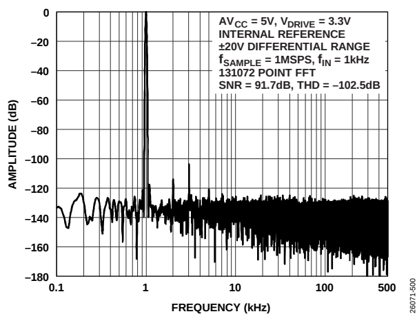
Figure 9. Fast Fourier Transform (FFT), \pm 20 V Differential Range, Low Bandwidth Mode
