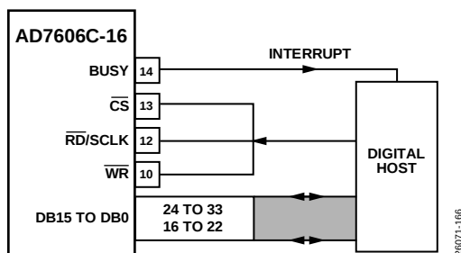
Figure 98. AD7606C-16 Interface Diagram—One AD7606C-16 Using the Parallel Bus with \overline{\text{CS}} and \overline{\text{RD}} Shorted Together
