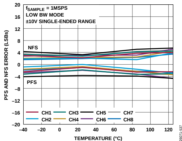
Figure 46. PFS and NFS Error vs. Temperature, \pm 10\text{ V} Single-Ended Range
