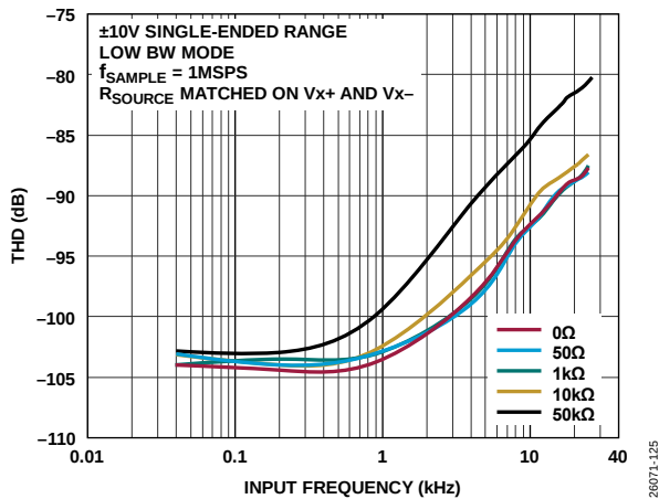
Figure 34. THD vs. Input Frequency for Various Source Impedances, \pm 10\text{ V} Single-Ended Range, Low Bandwidth Mode
