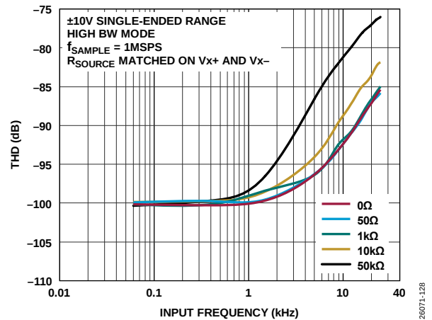
Figure 37. THD vs. Input Frequency for Various Source Impedances, \pm 10\text{ V} Single-Ended Range, High Bandwidth Mode
