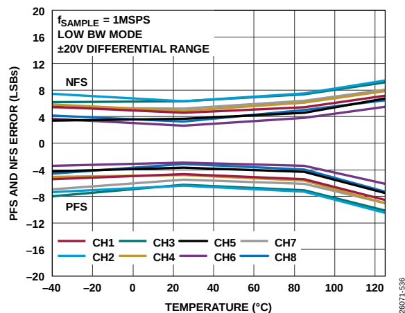
Figure 45. PFS and NFS Error vs. Temperature, \pm 20\text{ V} Differential Range
