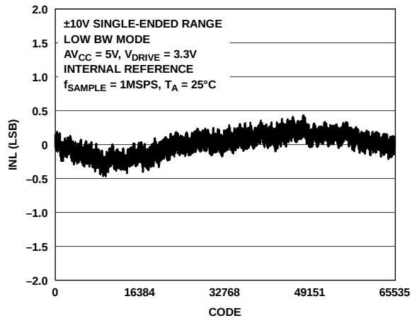
Figure 40. Typical INL, Low Bandwidth Mode
