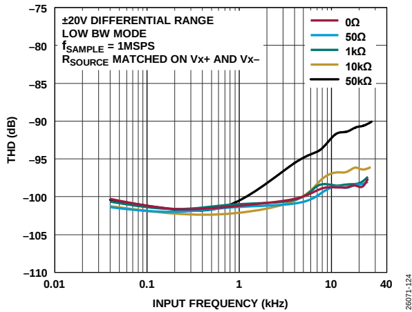
Figure 33. THD vs. Input Frequency for Various Source Impedances ( R_{\text{SOURCE}} ), \pm 20\text{ V} Differential Range, Low Bandwidth Mode
