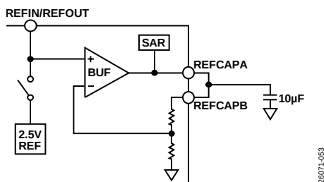
Figure 83. Reference Circuitry
