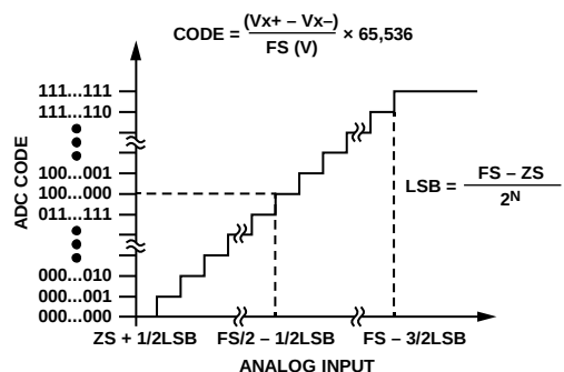
Figure 82. AD7606C-16 Ideal Transfer Characteristics, Unipolar Analog Input Ranges (Straight Binary Output Coding)
