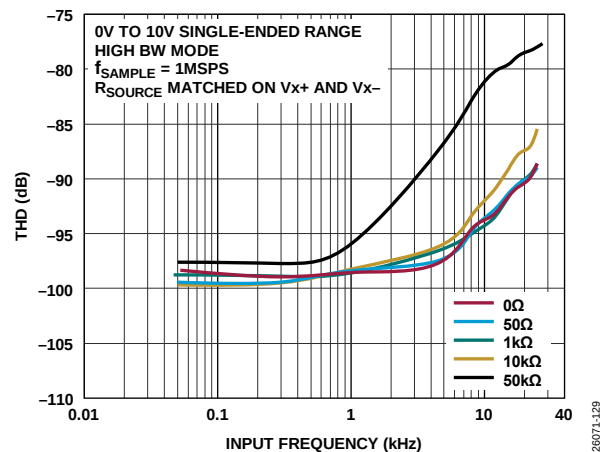
Figure 38. THD vs. Input Frequency for Various Source Impedances, 0\text{ V} to 10\text{ V} Single-Ended Range, High Bandwidth Mode
