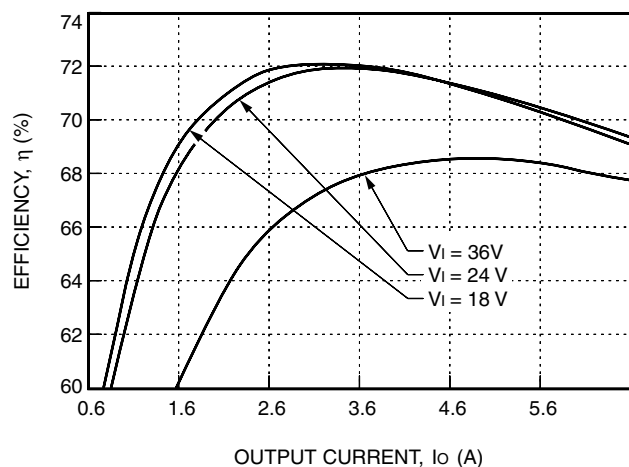
Figure 10. JC030D-M Typical Converter Efficiency vs. Output Current
