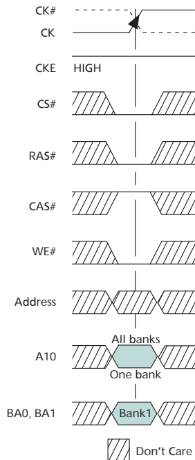
Figure 21: PRECHARGE Command
