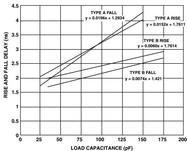
Figure 55. Typical Output Rise/Fall Delay Non-DDR ( V_{DD\_EXT} = \text{Max} )
