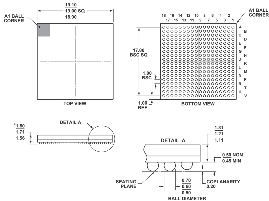
Figure 62. 324-Ball Chip Scale Package, Ball Grid Array [CSP_BGA] (BC-324-1) Dimensions shown in millimeters
