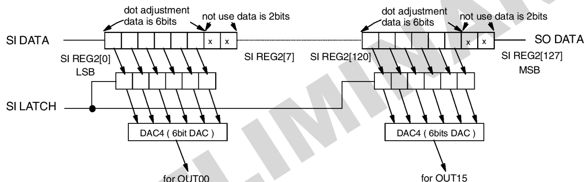
Figure 3-2 : the case of serial data transfer timing figure
