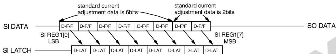
Figure 3-2 : the case of serial data transfer timing figure
