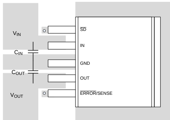
Figure 20. Layout Example for TO-263 Package
