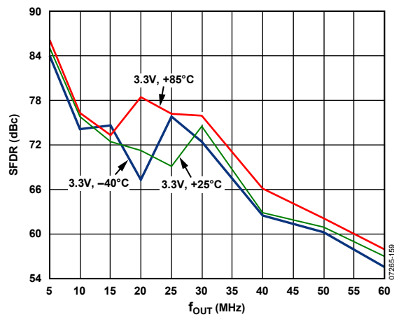
Figure 59. AD9717 SFDR at Three Temperatures, 3.3 V
