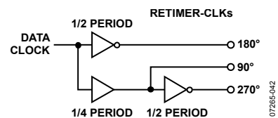
Figure 95. RETIMER-CLK Phases
