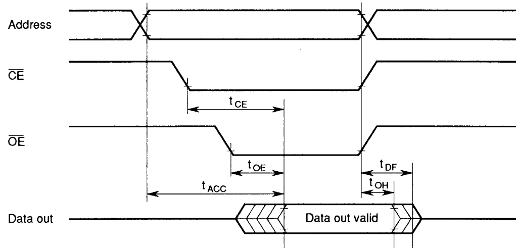
Figure 43 PROM Read Timing
