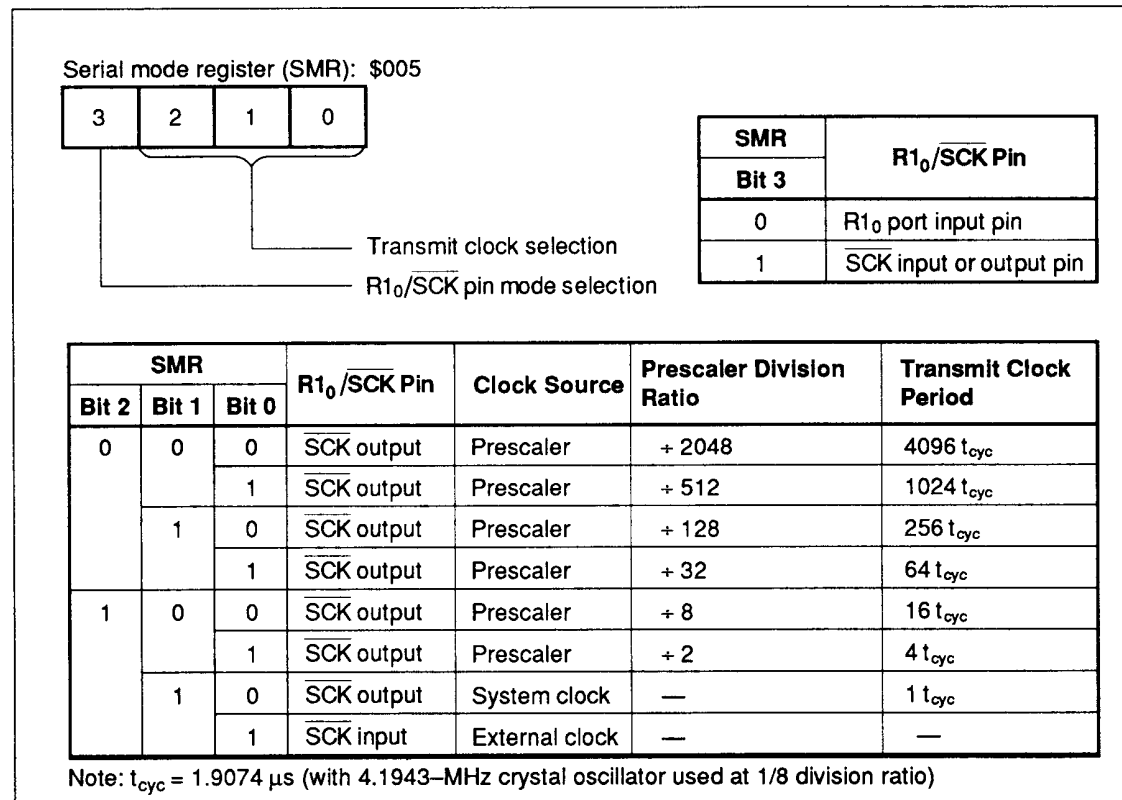
Figure 26 Serial Mode Register
