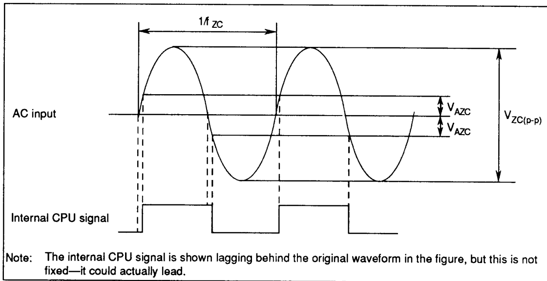
Figure 50 Zero-Crossing Detection
