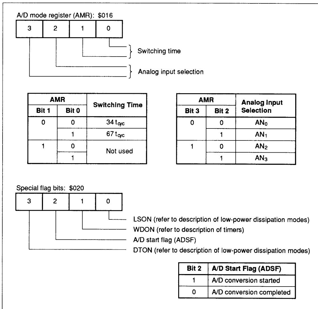
Figure 31 A/D Registers
