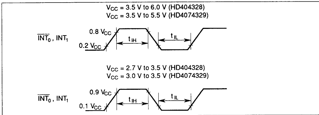
Figure 52 Interrupt Timing
