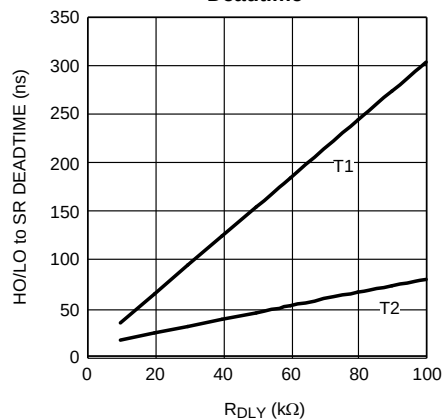
R_{DLY} vs Deadtime
