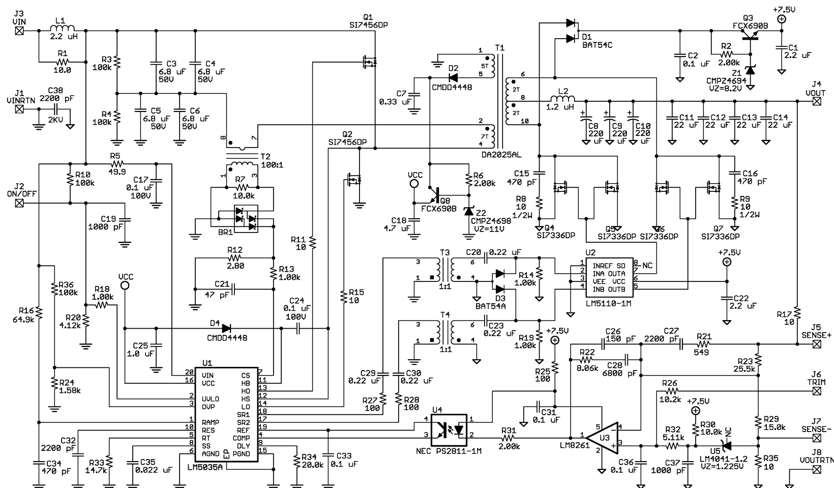
Figure 29. Evaluation Board Schematic
