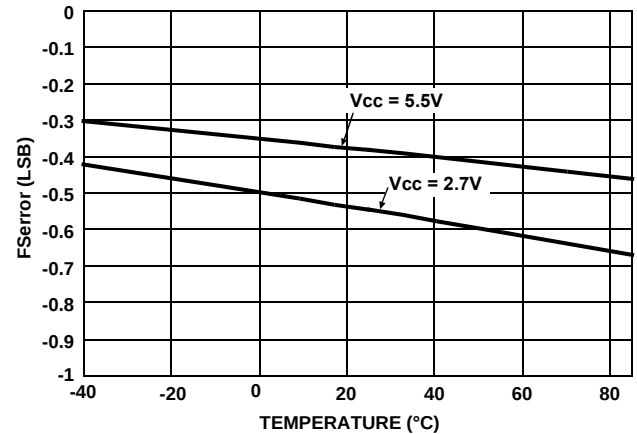
FIGURE 6. FError vs TEMPERATURE
