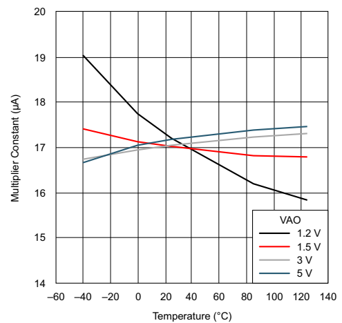
图 5-6. Multiplier Constant vs Junction Temperature
