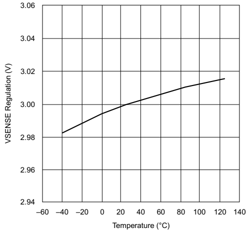
图 5-3. V_{VSENSE} Regulation vs Junction Temperature
