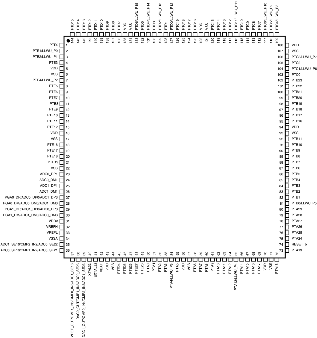
Figure 32. K10 144 LQFP Pinout Diagram
