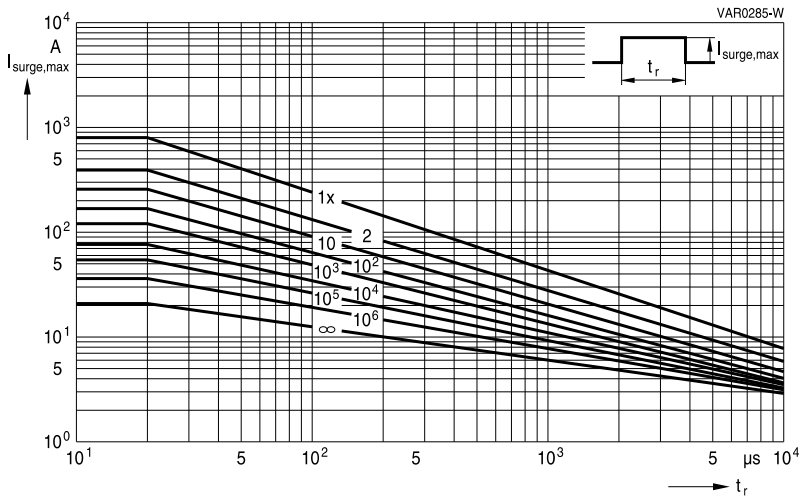
CN1812L8G ... K30G
