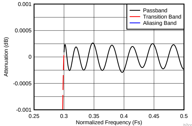
Figure 73. Decimate-by-2 Composite Zoomed Passband Response (D2_HIGH_PASS = 1)
