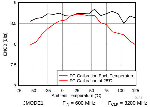
Figure 11. ENOB vs Temperature and Calibration Type
