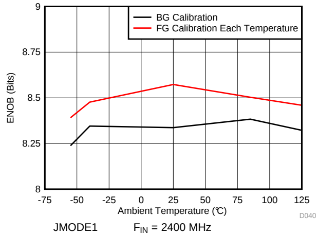
Figure 10. ENOB vs Temperature
