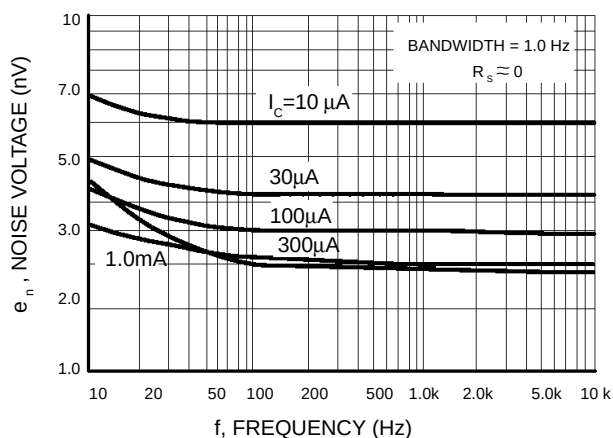
Figure 1. Noise Voltage
