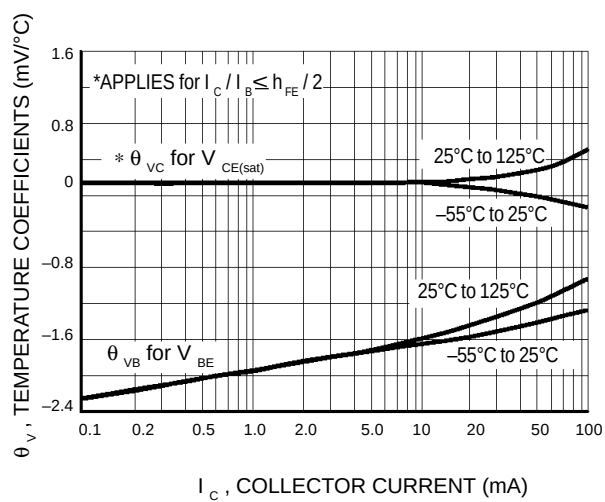
Figure 9. Temperature Coefficients
