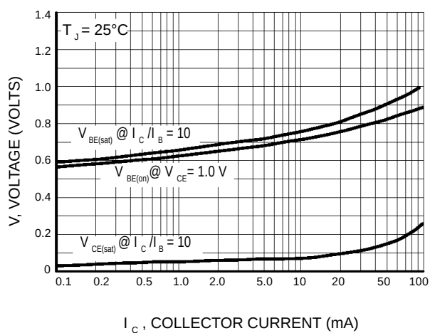
Figure 8. "On" Voltages
