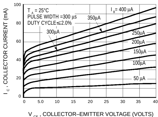
Figure 7. Collector Characteristics
