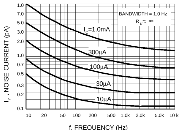
Figure 2. Noise Current
