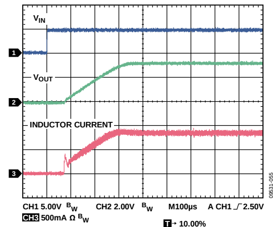
图55. 启动, V_{OUT} = 3.3\text{ V} , 800 mA
