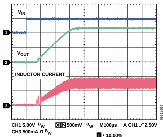
图57. 启动, V_{OUT} = 1.2V , 800 mA, V_{IN} = 5V
