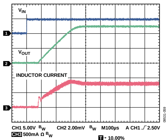
图59. 启动, V_{OUT} = 5V , 800 mA, V_{IN} = 7V
