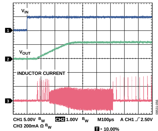
图56. 启动, V_{OUT} = 1.2\text{ V} , 10 mA, V_{IN} = 5\text{ V}
