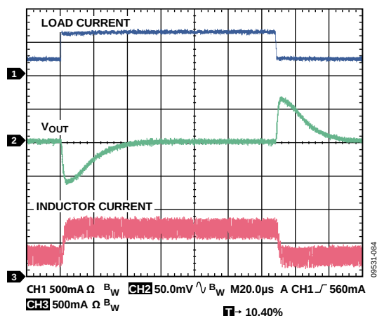
图84. 输出瞬态响应, V_{OUT2} = 1.8 \text{ V} , C_{OUT} = 10 \mu\text{F} , 300 mA至800 mA, 负载电流上升时间 = 200 ns
