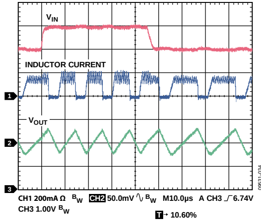
图34. 线路瞬态响应, V_{OUT} = 5 V, PSM模式, 100 mA, V_{IN1} = 6 V至7 V, 2\mu s上升时间, C_{IN} = 3.3\mu F
