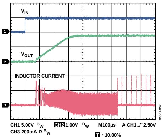
图52. 启动, V_{OUT} = 1.8\text{ V} , 10 mA
