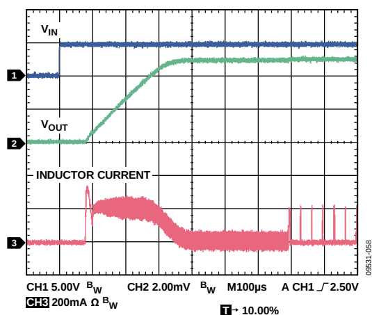
图58. 启动, V_{OUT} = 5V , 10 mA, V_{IN} = 7V
