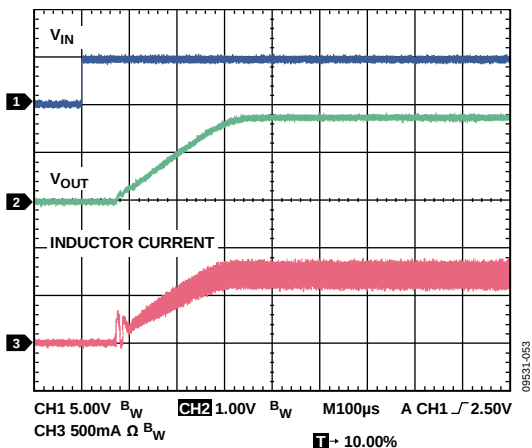
图53. 启动, V_{OUT} = 1.8\text{ V} , 800 mA
