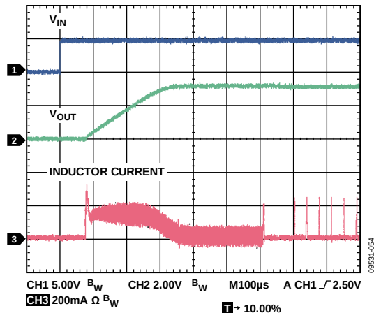
图54. 启动, V_{OUT} = 3.3\text{ V} , 10 mA
