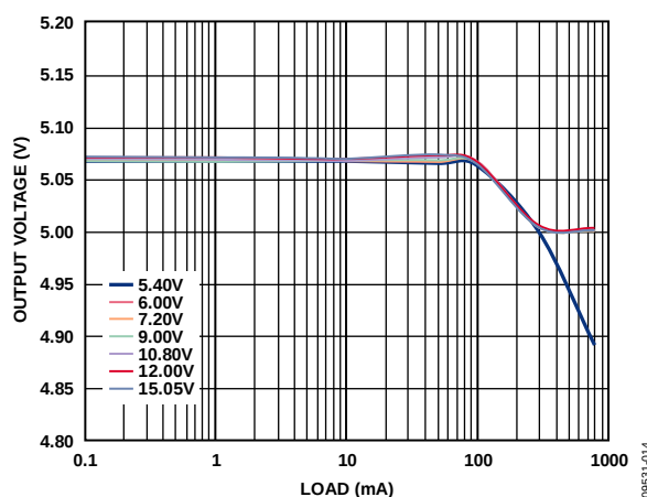
图14. 负载调整率, V_{OUT} = 5.0\text{ V}
