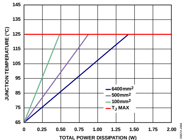
图88. 结温与功耗的关系, T_A = 65^\circ\text{C}
