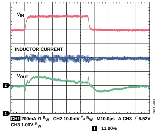
图35. 线路瞬态响应, V_{OUT} = 5 V, PWM模式, 800 mA, V_{IN1} = 6 V至7 V, 2\mu s上升时间, C_{IN} = 3.3\mu F
