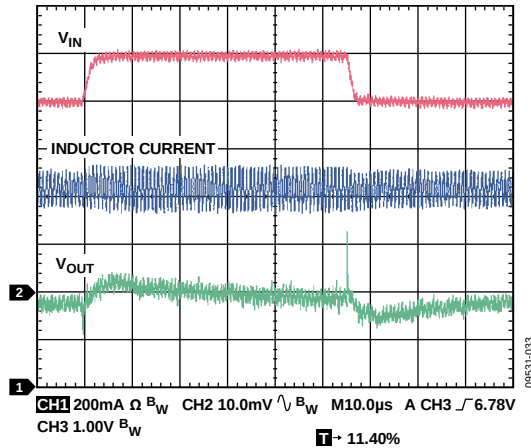
图33. 线路瞬态响应, V_{OUT} = 3.3 V, PWM模式, 800 mA, V_{IN1} = 6 V至7 V, 2\mu s上升时间, C_{IN} = 3.3\mu F
