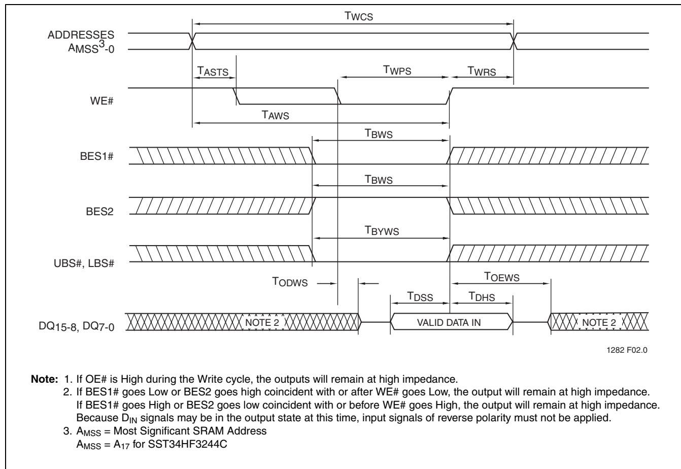
FIGURE 5: SRAM Write Cycle Timing Diagram ( \text{WE}\# Controlled)
