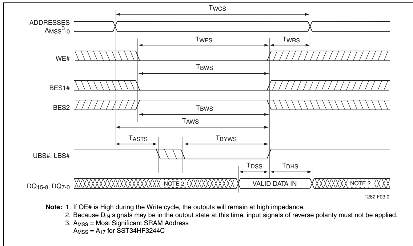
FIGURE 6: SRAM Write Cycle Timing Diagram (UBS#, LBS# Controlled)
