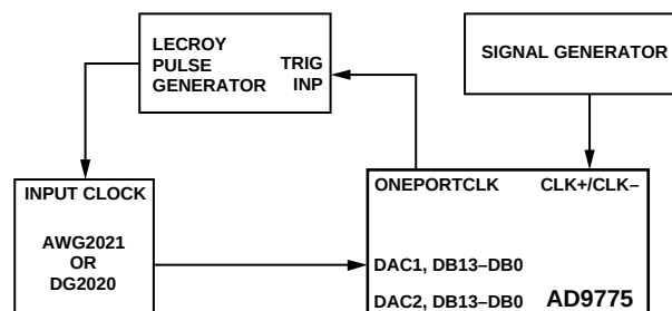
Figure 101. Test Configuration for AD9775 in Two-Port Mode with PLL Enabled, Signal Generator Frequency = Input Data Rate, DAC Output Data Rate = Signal Generator Frequency \times Interpolation Rate
