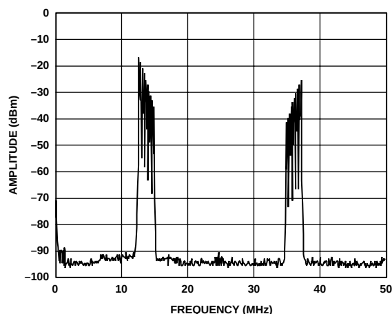
Figure 91. AD9775 Real DAC Output of Complex Input Signal Near Baseband (Positive Frequencies Only), Interpolation = 4\times , Complex Modulation in AD9775 = +f_{DAC}/4
