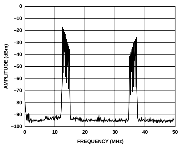
Figure 93. AD9775 Real DAC Output of Complex Input Signal Near Baseband (Negative Frequencies Only), Interpolation = 4\times , Complex Modulation in AD9775 = -f_{DAC}/4
