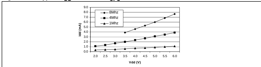
Figure 60. Typical I_{DD} in RUN vs. f_{CPU}
