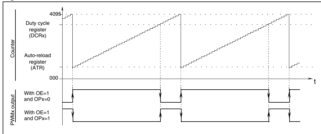
Figure 36. PWM function
