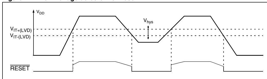
Figure 17. Low voltage detector vs. Reset
