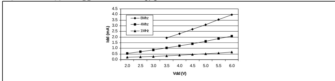
Figure 62. Typical I_{DD} in WAIT vs. f_{CPU}
