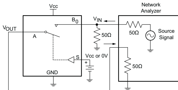
Figure 5. Off Isolation
