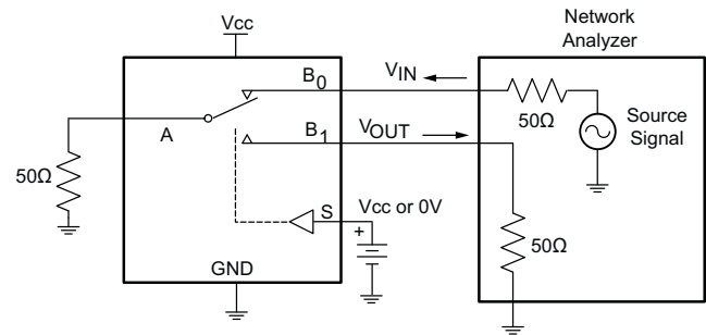
Figure 6. Crosstalk
