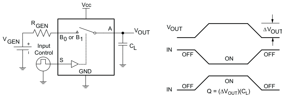
Figure 8. Charge Injection
