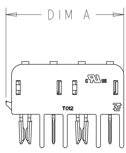
2213288-2/ 1-2213288-2 SCALE 3:1
