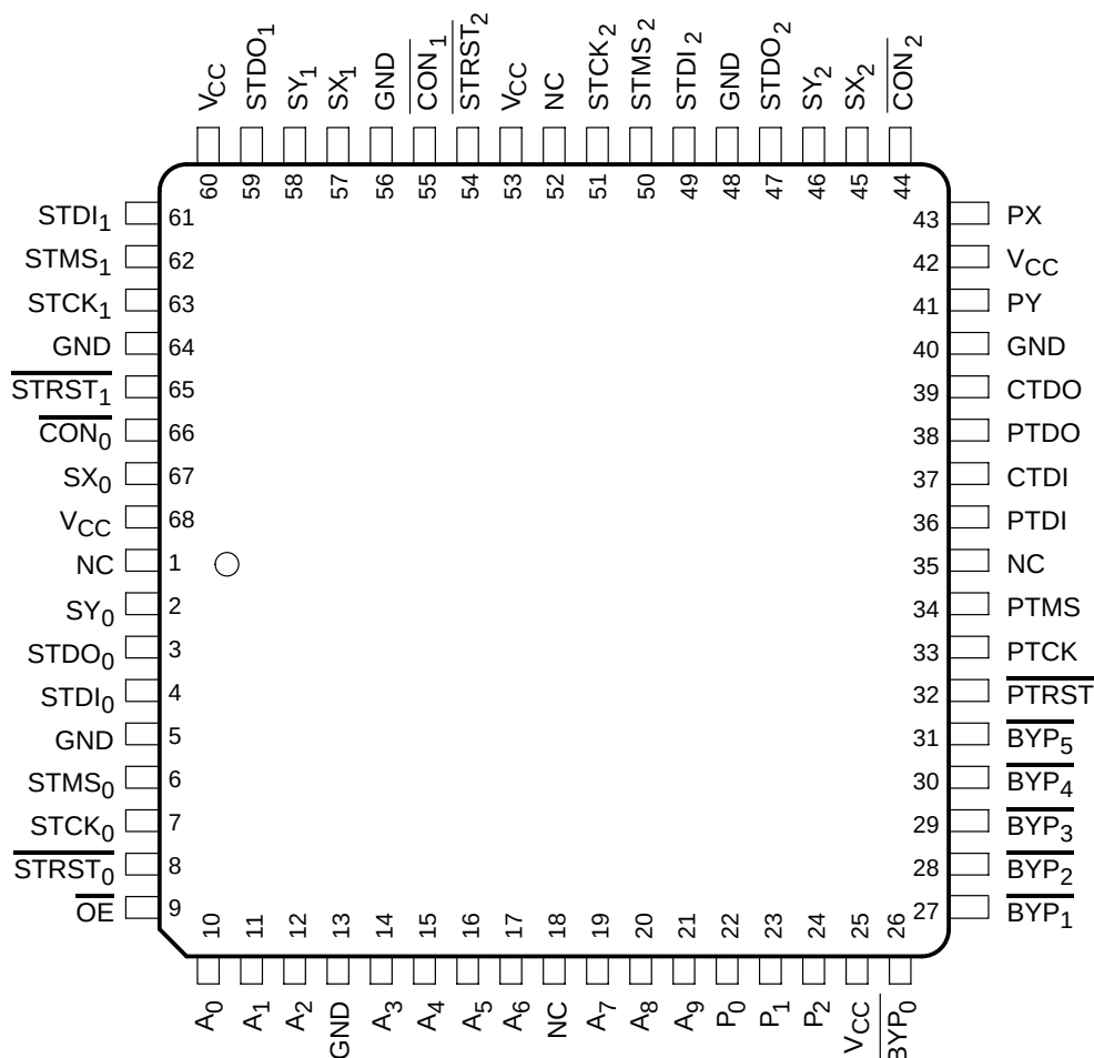
SN54LVT8986 . . . HV PACKAGE (TOP VIEW)
