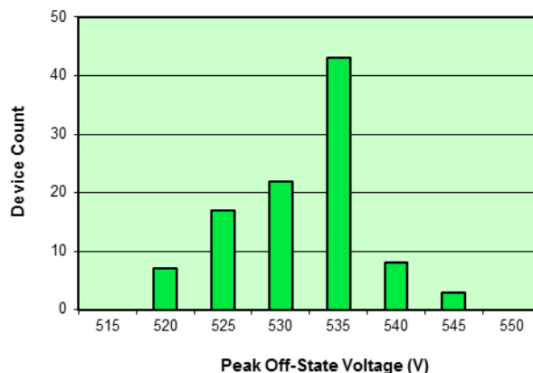
Figure 2: Typical Peak Off-State Voltage Distribution ( N = 100 , T_A = 25^\circ\text{C} )
