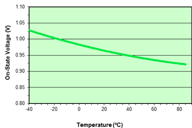
Figure 5: Typical LED Voltage vs Temperature
