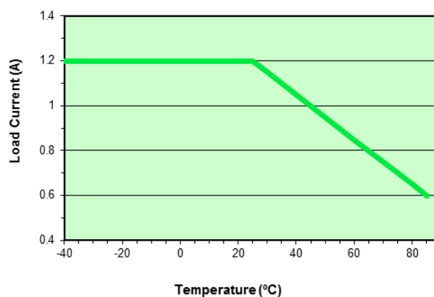
Figure 4: Maximum Load Current vs. Temperature
