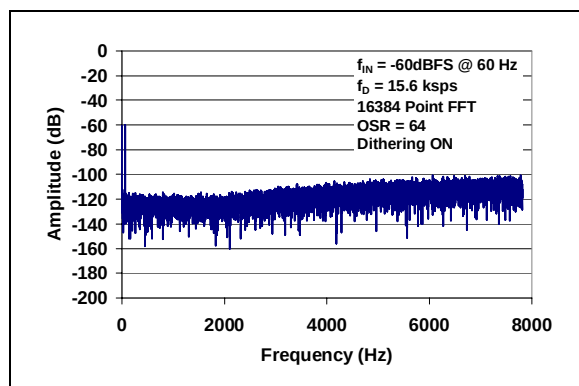
FIGURE 2-8: Spectral Response.
