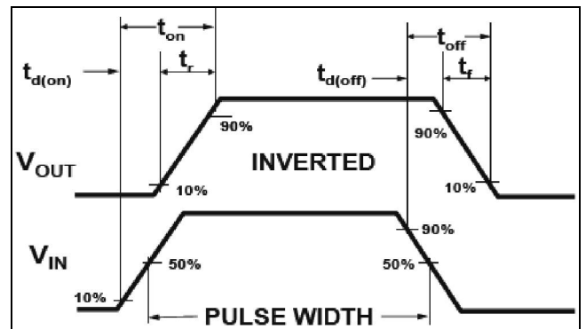
Switch Waveform
