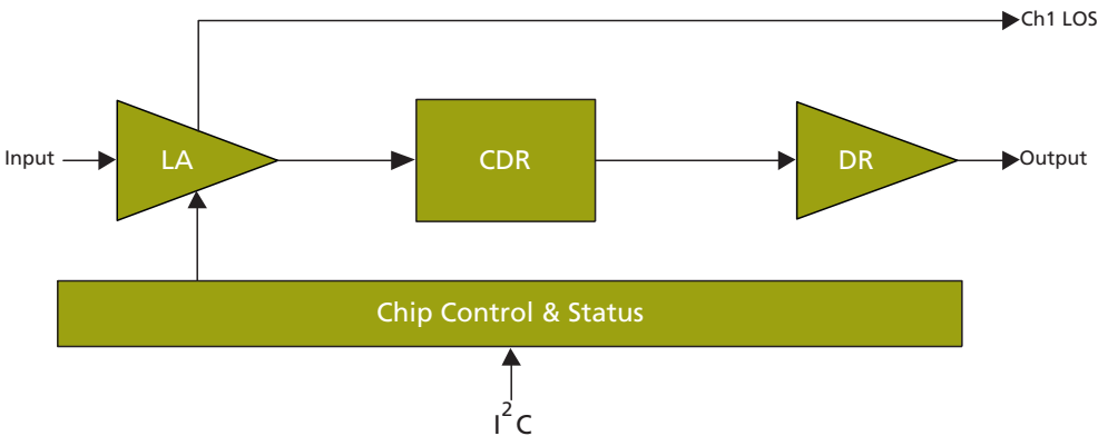
Figure 3-2: Channel 1 Path
