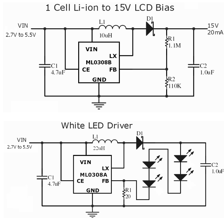
Figure 1: One-cell Li-ion to 15V Converter and White LED Driver
