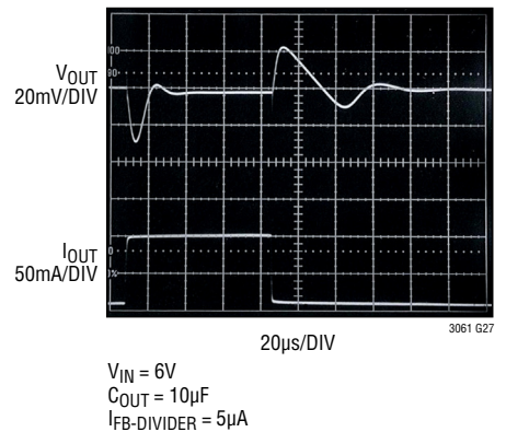
5V Transient Response C_{FF} = 10\text{nF} , I_{OUT} = 10\text{mA} to 100\text{mA}
