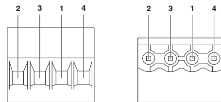
Pin assignment left
