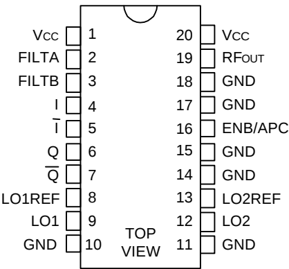
Figure 2. Pin Diagram
