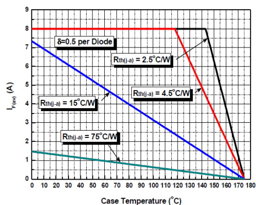
Figure 4. Current Derating Curves
