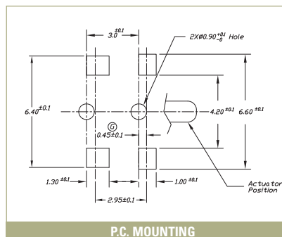
P.C. MOUNTING
