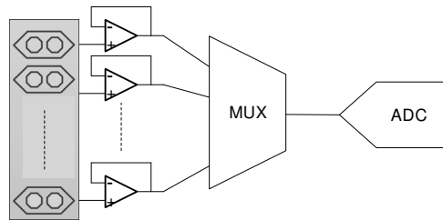
图 9-16. Multichannel Sensor Interface Using Multiple Amplifiers
