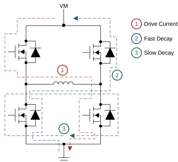
Figure 14. Decay Modes
