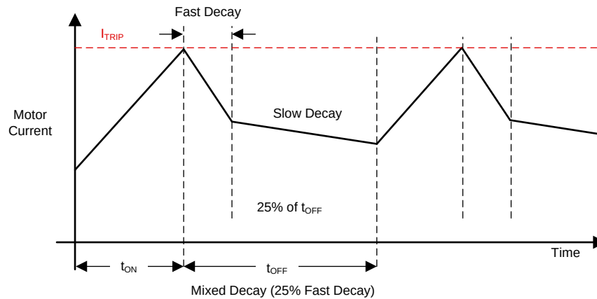
Figure 15. Mixed Decay
