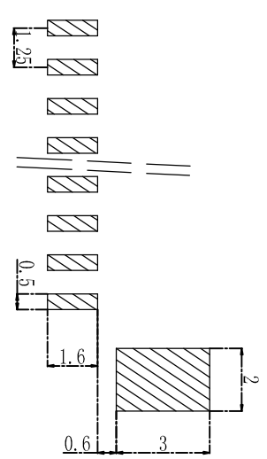
PCB尺寸 PCB Layout
