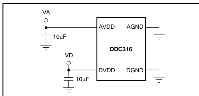
Figure 18. Power-Supply Connections
