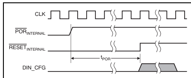
Figure 17. Power-Up Timing
