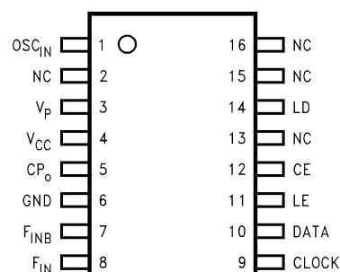
16-Pin TSSOP Package NS Package Number MTC16
