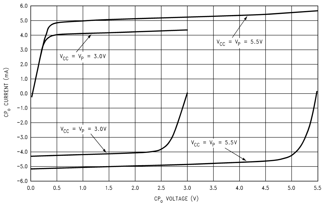
LMX2346/7 Charge Pump Sweeps
