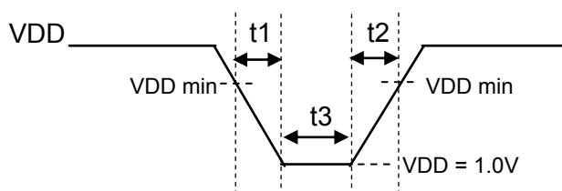
Figure 45. VDET Detection Timing
