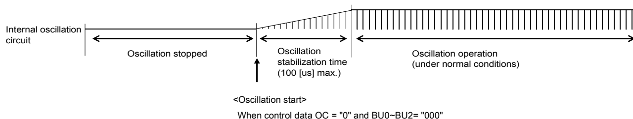
Figure 44. Oscillation Stabilization Time
