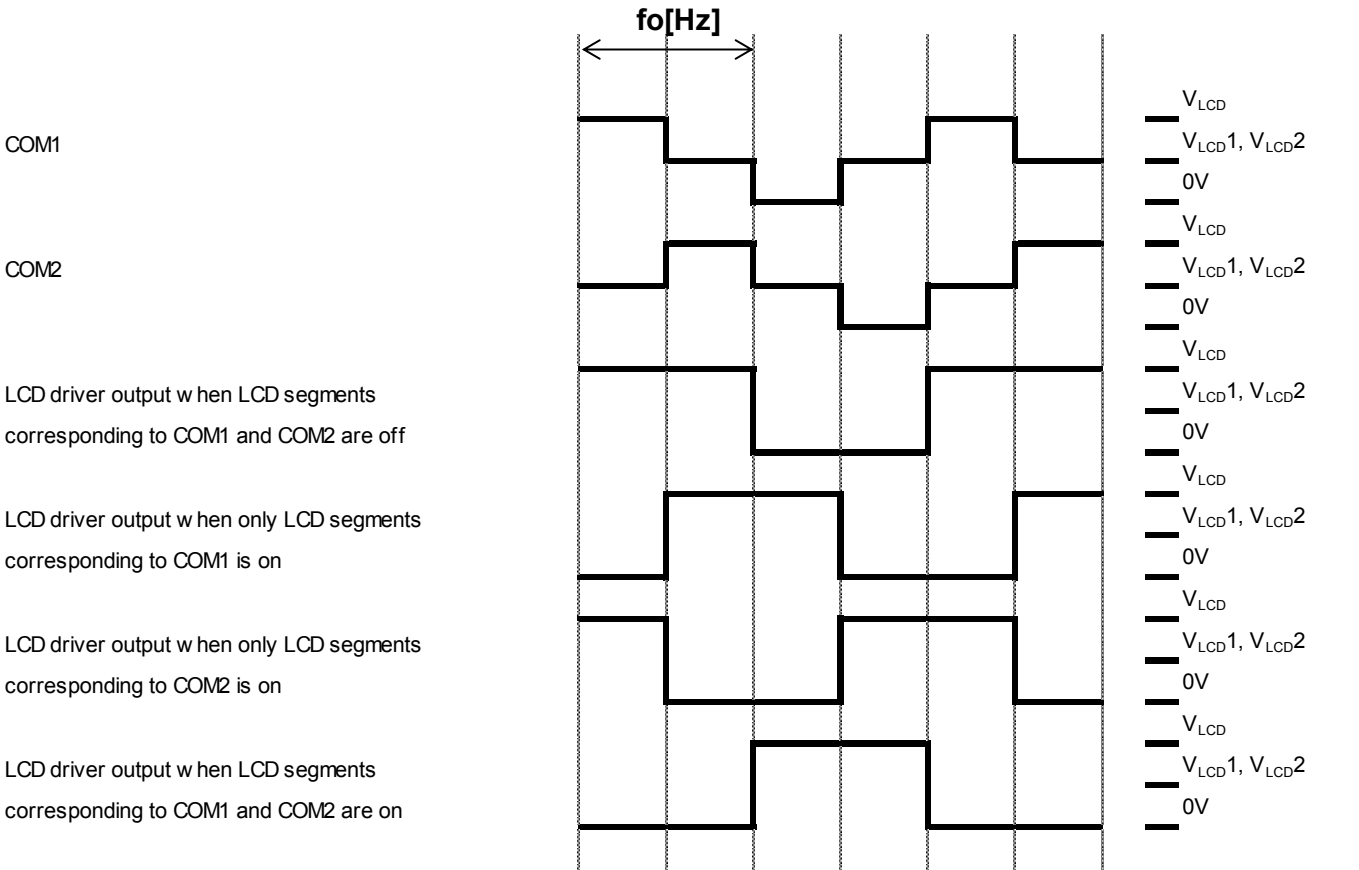
Figure 38. LCD Waveform (Frame Inversion, 1/2 DUTY, 1/2 BIAS) (Note)
