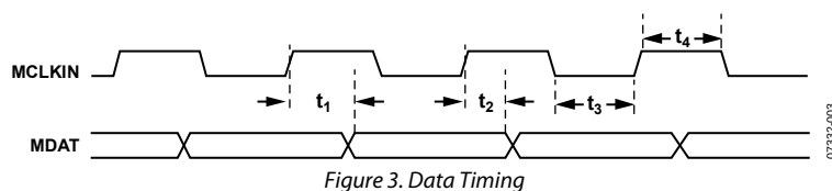
Figure 3. Data Timing
