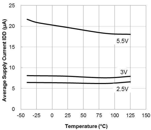
Average Supply Current vs. Temperature
