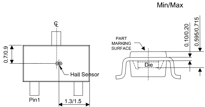
Sensor Location
