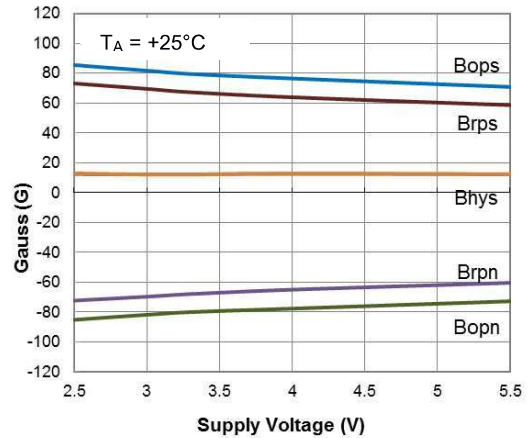
Switch Points vs Supply Voltage
