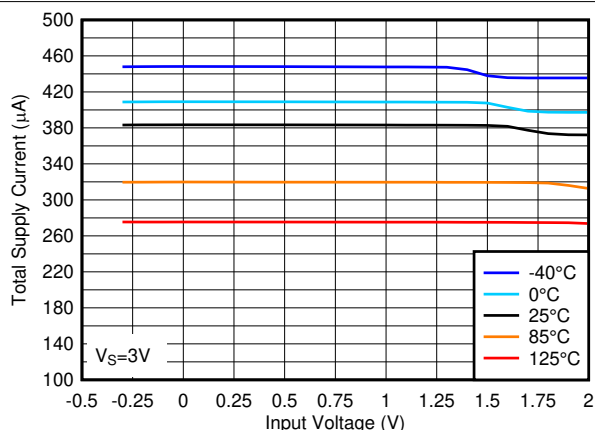
图 3-8. Total Supply Current vs. Input Voltage at 3V
