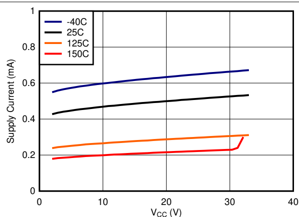
图 3-2. Supply Current vs. Supply Voltage LM2903E-Q1 Only
