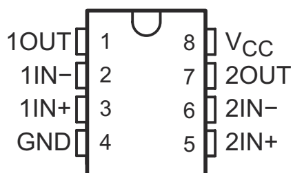
图 2-1. D, DGK, DDF OR PW PACKAGE Top View
