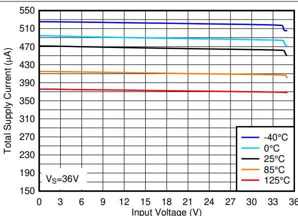
图 3-12. Total Supply Current vs. Input Voltage at 36V
