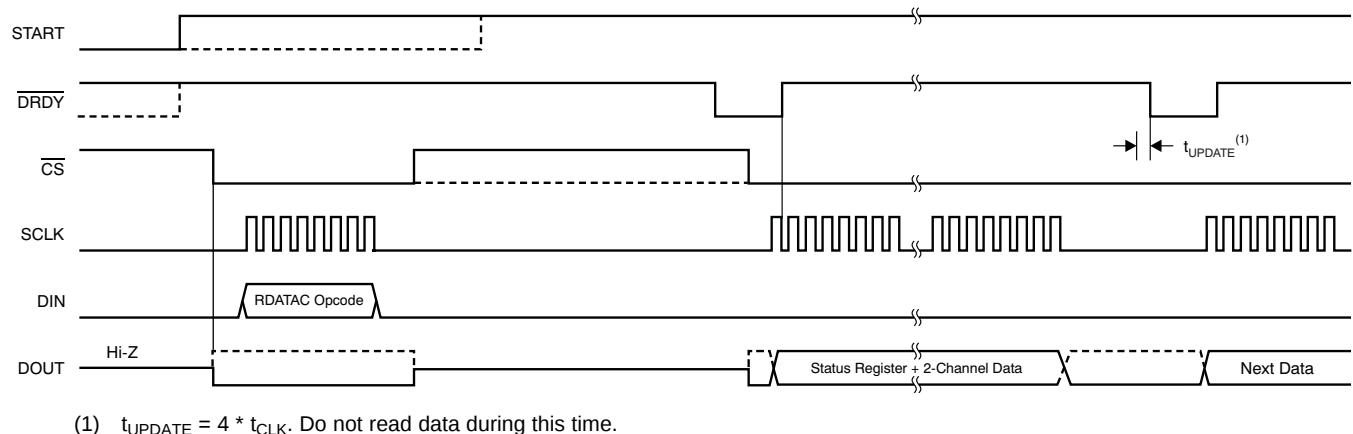
Figure 38. RDATAAC Usage
