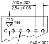
RECOMMENDED PC BOARD LAYOUT
