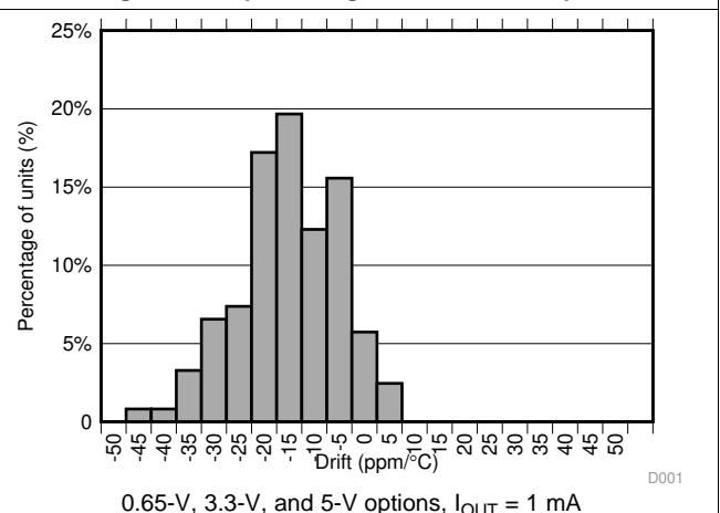
Figure 4. Temperature Drift Histogram (-40°C to +25°C)
