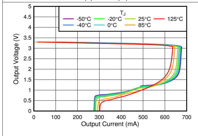
Figure 29. 3.3-V V_{OUT} vs I_{OUT}
