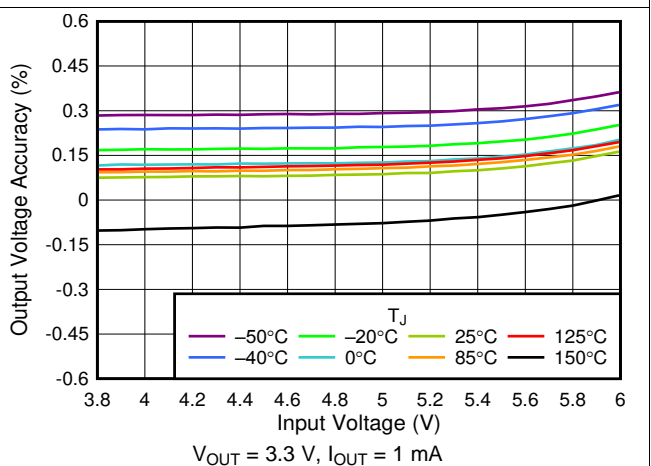
Figure 6. 3.3-V Line Regulation vs V_{IN}
