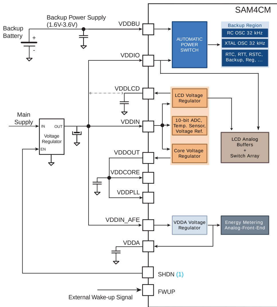
Figure 5-3. Single Supply Operation with Backup Battery
