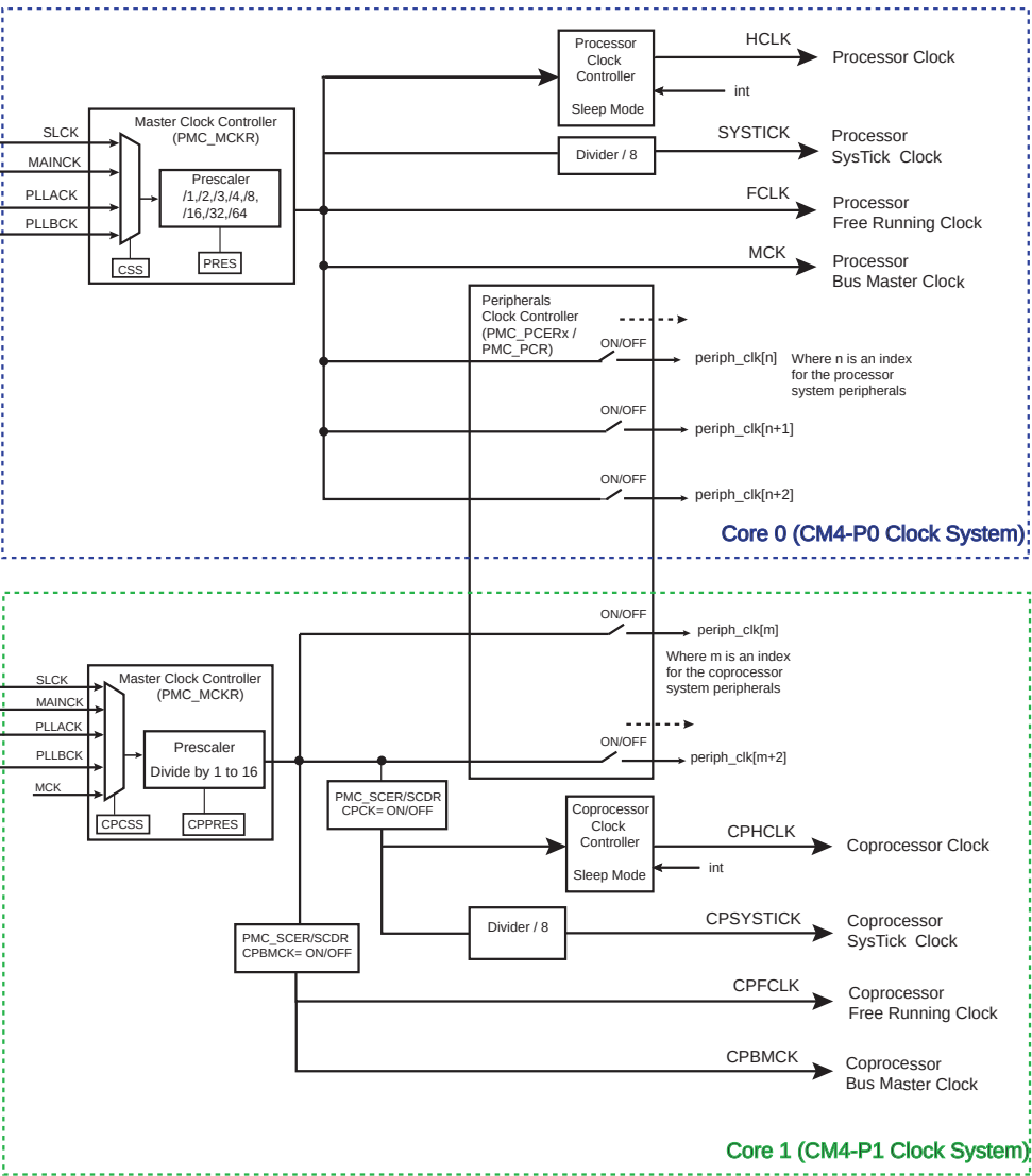
General Clock Block Diagram
