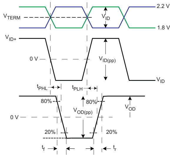
Figure 20. TMD5 Main Link Timing Measurements
