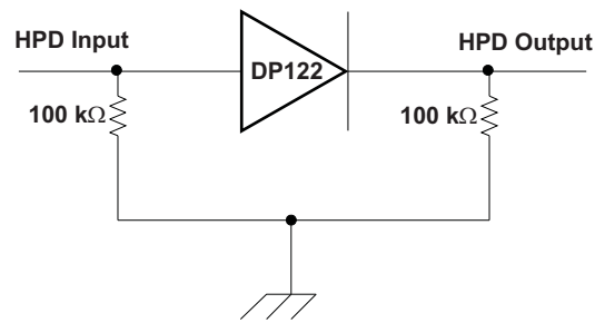
Figure 1. HPD Test Circuit
