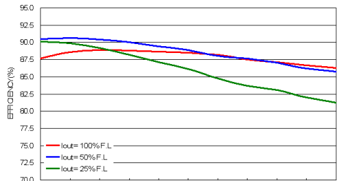
WAF(D)150-48S24W Efficiency vs. Input Voltage
