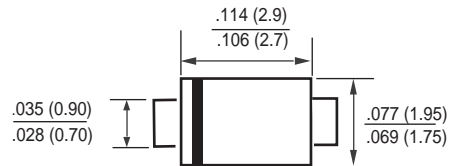
SOD-123F
