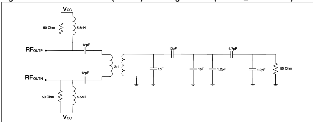
Figure 30. Evaluation Board (EVB4G) matching network (MATCH_EVB4G.dsn)
